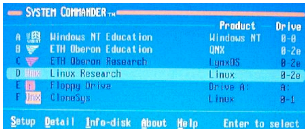
Figure 2: System Commander boot screen as used in Patagonia-Cluster at ETH Zürich.
