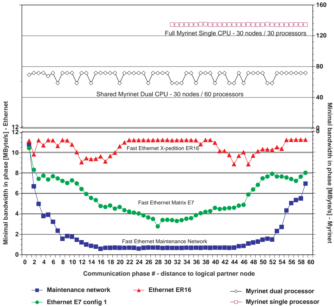
Figure 10: All-to-all minimal per-node bandwidth for different communication phases for all the discussed network architectures.
