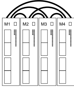
Figure 6: Matrix E7 and ER16 backplane: All line modules are connected with all other modules. The backplane itself should not be a limitation to the total communication bandwidth.
