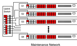
Figure 1: The maintenance network configuration has a very limited bisection bandwidth since 16 nodes (connected by Fast Ethernet) share a single Fast Ethernet up-link.
