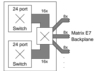
Figure 5: Matrix E7 module: Each module consists of two internal 24 port switches that are able to communicate at full speed to each other or with reduced speed to the E7 backplane.
