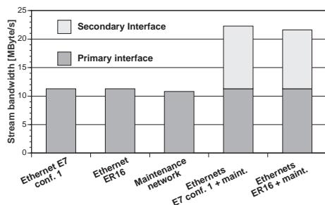
Figure 12: Average bandwidth of Dolly stream through 30 nodes with the full bisection Ethernet with the configuration 1 and maintenance network alone as well as combined.
