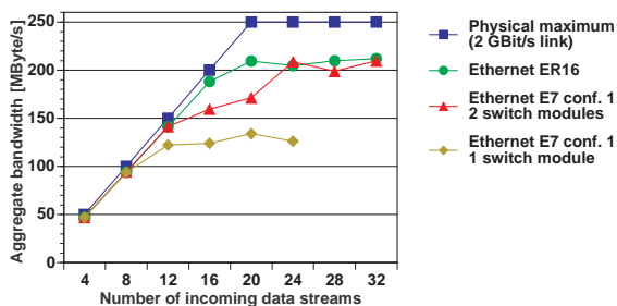
Figure 7: Aggregate bandwidths for increasing numbers of data streams transmitted into the Xibalba cluster.
