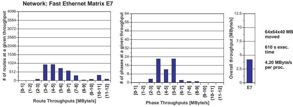
Figure 3: Histograms of transfer rates for the 64^2 routes (left), the transfer rates of the 64 phases (right) and the overall performance in a phased AAPC algorithm on a 64 processor cluster for the E7 network configuration.
