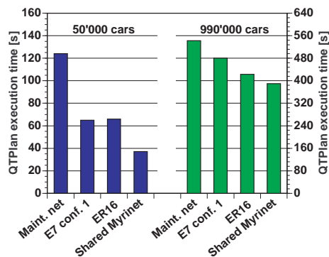
Figure 14: Runtime of QTPlan traffic simulations for 50'000 and 990'000 cars on 64 nodes/processors in seconds.
