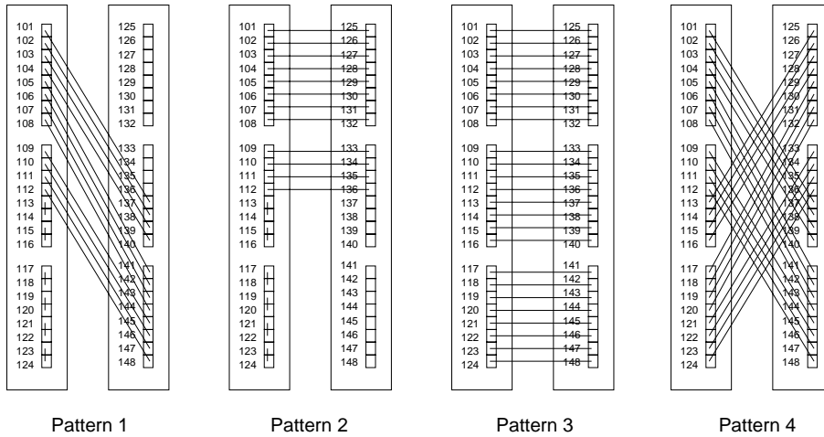
Figure 8: Test pattern used to evaluate the ER16 switch. Pattern 1 leads to reduced bisection in the full bisection network whereas patterns 2–4 work well.
