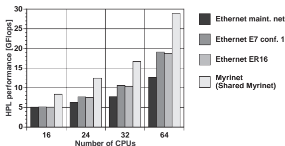
Figure 13: Performance comparison of cheap, medium and expensive networking architectures for the HPL benchmark in GFlops.
