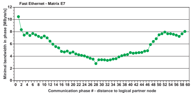
Figure 2: All-to-all performance for different communication phases for the Enterasys Matrix E7 Switch.
